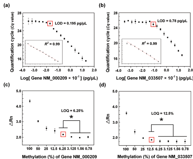
Fig. 2 LOD and LOQ for the qPCR-based MethyLight assay using standard DNA samples. (a) The LOD for gene NM_000209 is 0.195 \text{ pg } \mu\text{L}^{-1} . (b) The LOD for gene NM_033507 is 0.78 \text{ pg } \mu\text{L}^{-1} . (c) and (d) The LOQ was 6.25% for gene NM_000209 and 12.5% for gene NM_033507, respectively ( p < 0.05 ) ( \Delta R_n means normalized reporter signal).
