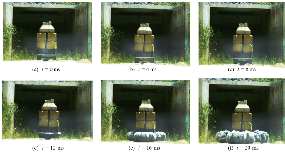
Figure 8 (Color online) Sequential expanding processes of sand subjected to detonation of shallow-buried explosive.
