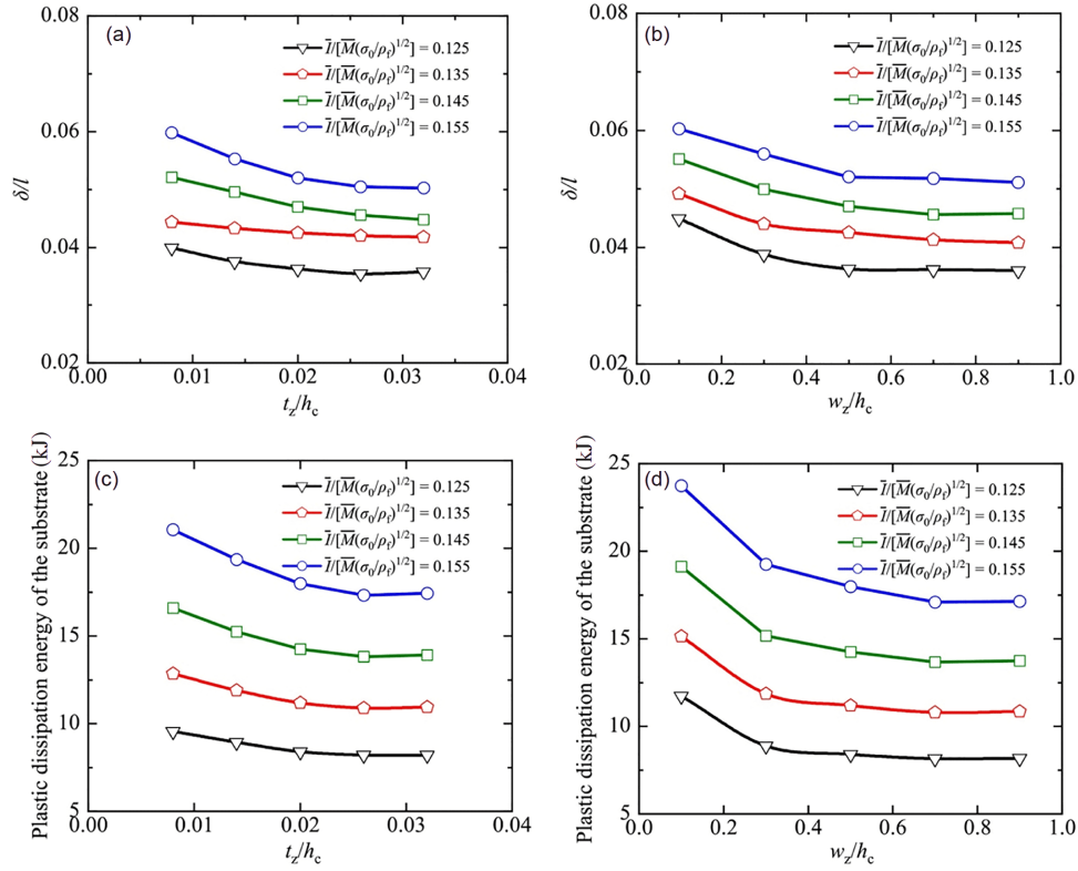
Figure 29 (Color online) Residual deformation of steel substrate plotted as a function of (a) normalized thickness and (b) normalized width of z-tubes, and plastic dissipation energy of steel substrate plotted as a function of (c) normalized thickness and (d) normalized width of z-tubes.
