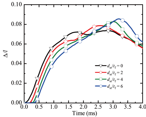
Figure 20 (Color online) Midpoint displacement of steel substrate plotted as a function of time for selected gap thicknesses between substrate and sandwich panel, with I / [\overline{M}(\sigma_0/\rho_f)^{1/2}] = 0.155 .
